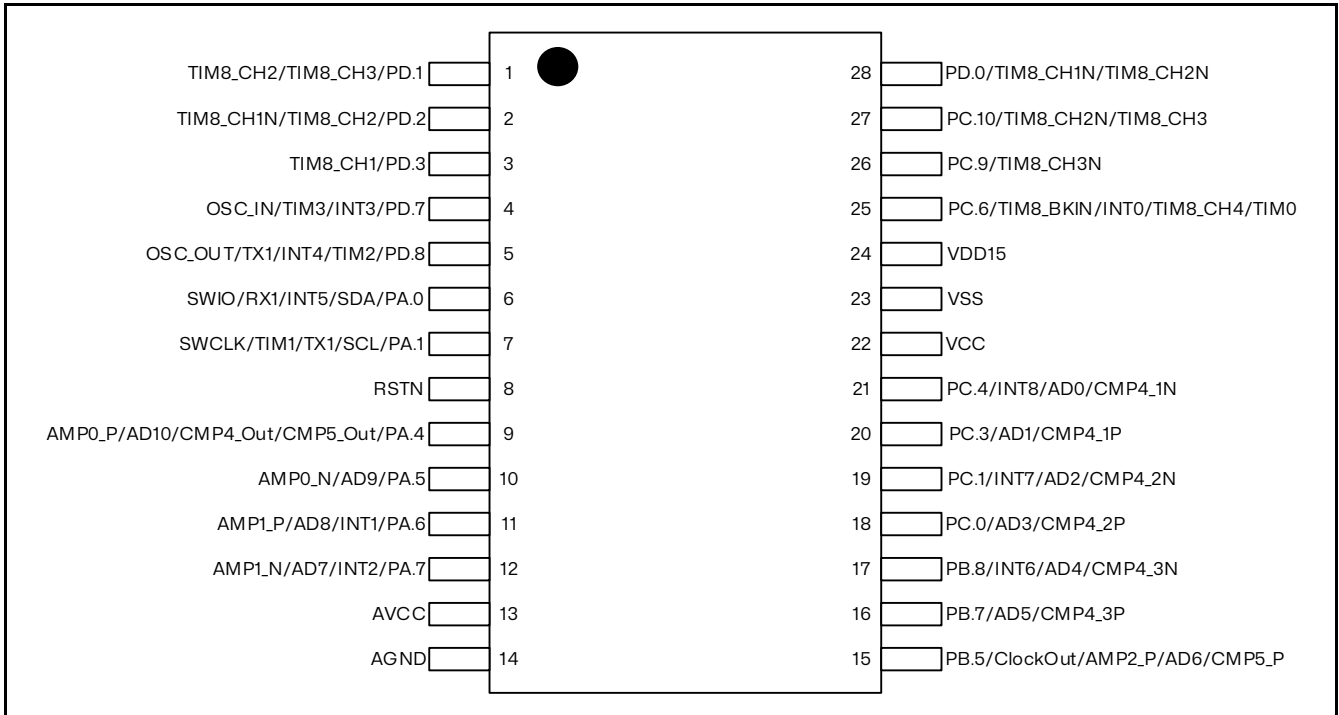
Figure 4.1 RX32S11 TSSOP28 package pinout
