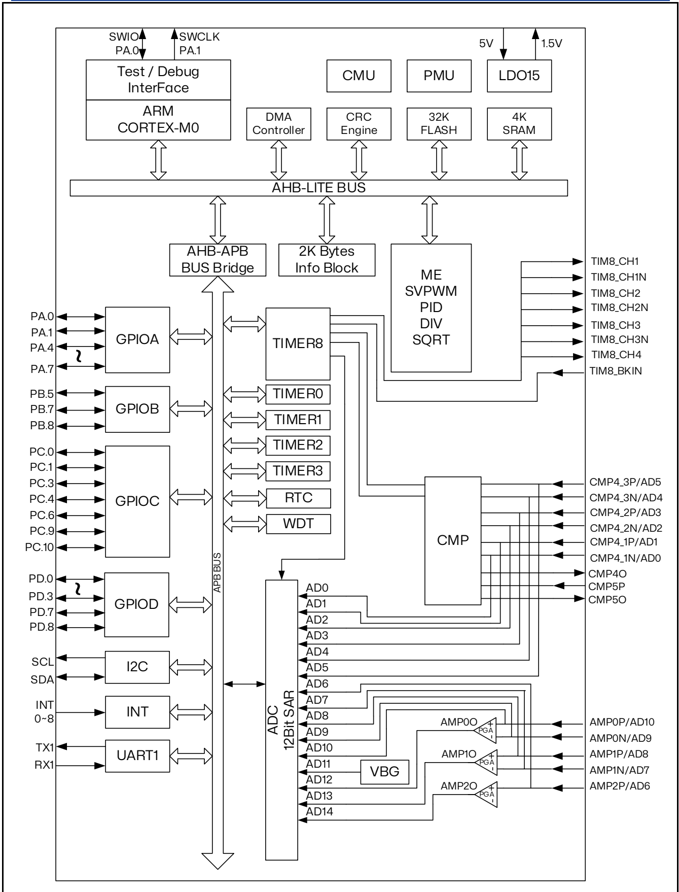
Figure 2.1 RX32S11 Block diagram
