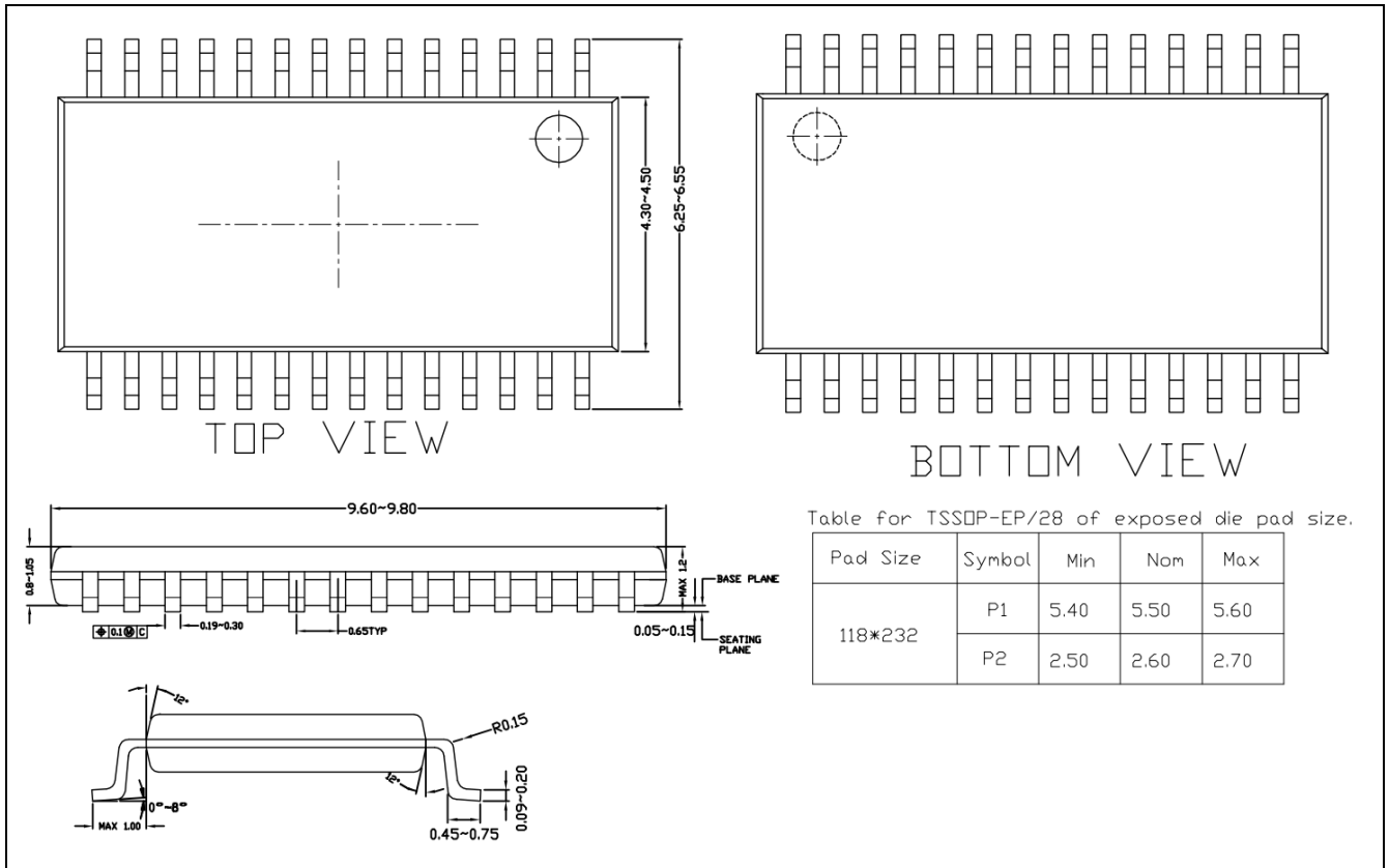
Figure 6.1 TSSOP28 package outline
