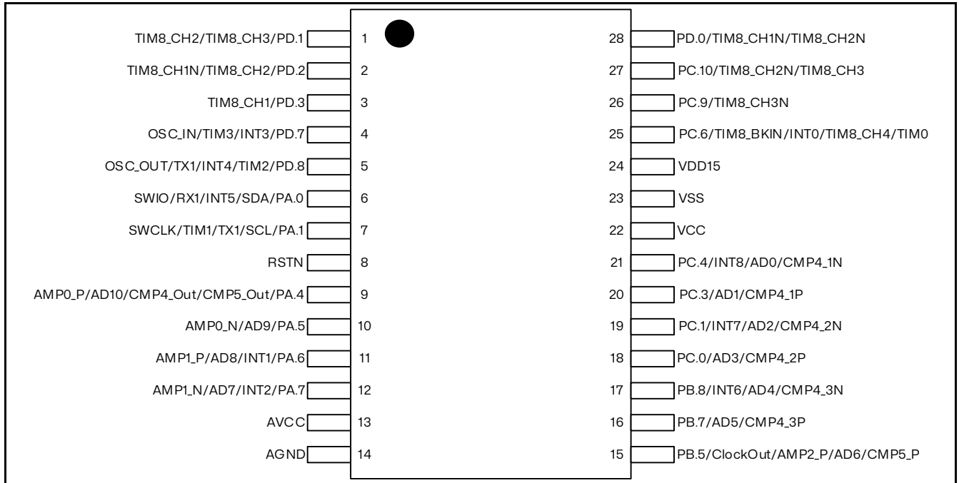
Figure 4.1 RX32S11 TSSOP28 package pinout
